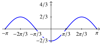
Figure 1. The indicator function h of \text{Ai} .
