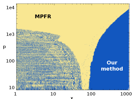
Figure 3. Fastest method as a function of x and p (scales are logarithmic).
