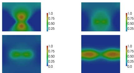
Figure 3. Cathode break: evolution of the transmembrane potential u after the turnoff of the cathode for the current lifted monodomain model (endocardial surface is shown at times 2, 6, 10, 25 ms).
