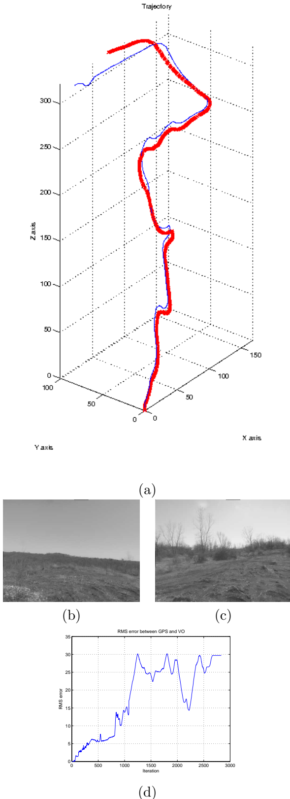
Fig. 12. The outdoor Dunes sequence taken from a ground vehicle with (a) GPS ground truth data in blue and the visual odometry estimation in red. (b) and (c) show two images from this difficult sequence. (d) The RMS error in meters between the GPS and visual sensors, it can be seen that there is significantly more drift when there are large rotations at iterations anti-clockwise from 1081 to 1244 and clockwise from 1996 to 2121.
