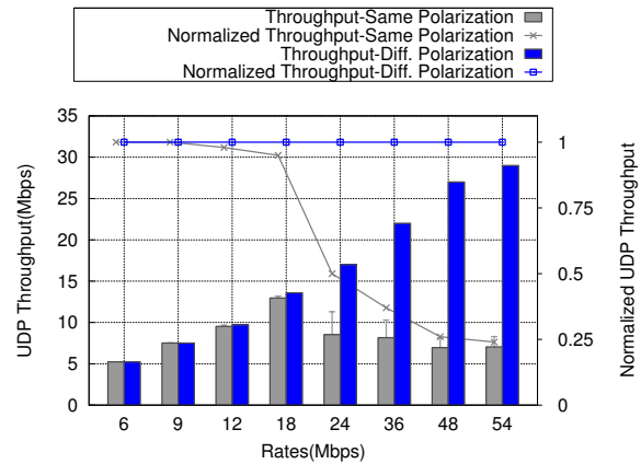
Fig. 5. Received UDP throughput as a function of different bit-rates when antenna separation is fixed at 6cm and power level of the interfering transmit interface on 2.4GHz is set to 17dBm.
