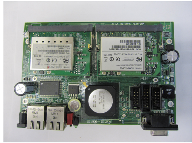
Fig. 1. Gateworks Avila multi-radio platform equipped with two Compex WLMAG54-23dBm mini PCI cards.
