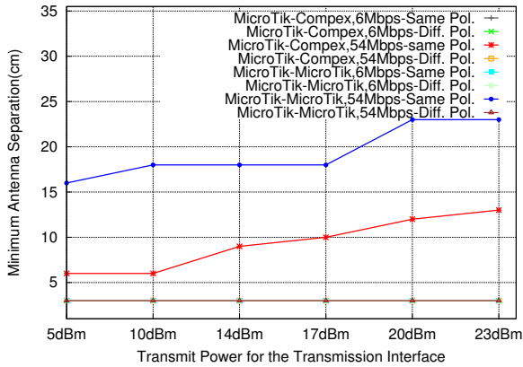
Fig. 4. Impact of using a different radio interface card and different radio interface cards in combination on minimum antenna separation required to avoid throughput degradation on Avila based dual-radio 802.11 platform at different bit-rates, antenna polarizations and collocated interferer transmit power levels.
