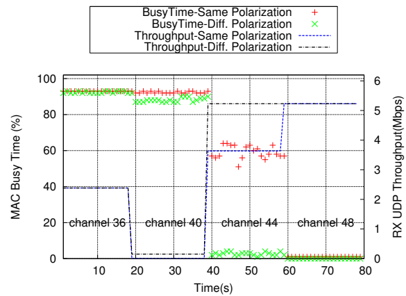
Fig. 7. The effect of adjacent channel interference (ACI) on receive MAC BUSY time and throughput at different channel separations and polarizations between collocated interfaces.
