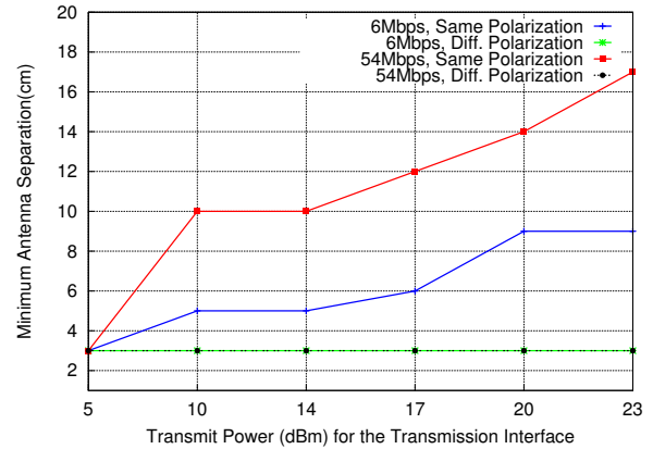
Fig. 3. Minimum antenna separation required to avoid throughput degradation on Avila based dual-radio 802.11 platform at different bit-rates, antenna polarizations and collocated interferer transmit power levels.
