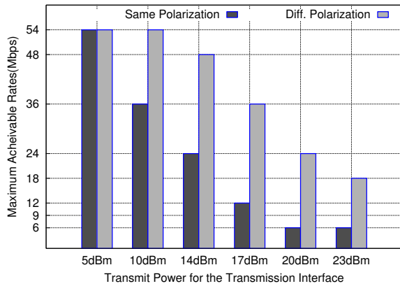
Fig. 6. Maximum achievable bit-rates on the receive interface at different power levels for the transmit interface when both interfaces are tuned to far apart channels within the 5GHz and their antennas are separated by 40cm.
