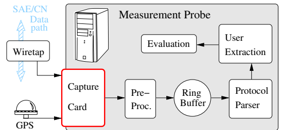
Fig. 3. Detail of the measurement probes within the mobile networks. The probes timestamp captured packets and decode them for identification and packet-matching.
