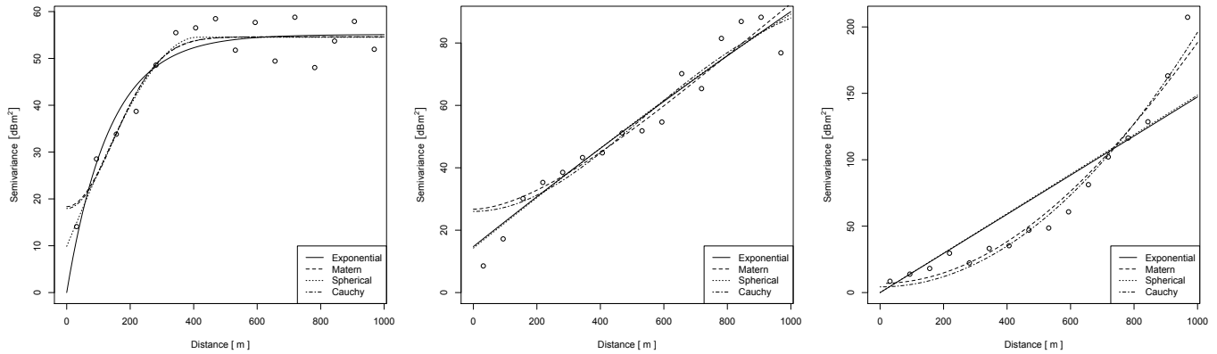
Fig. 5. Semivariogram fits for the operator A (left), B (middle) and C (right) data sets.
