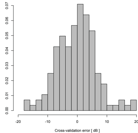
Fig. 7. The distribution of cross-validation errors for operator A data set.
