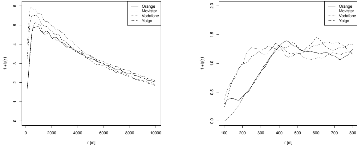
Fig. 2. The pair correlation function estimates for the UMTS cellular network sites in suburbs (left) and downtown Madrid (right) for different operators.
