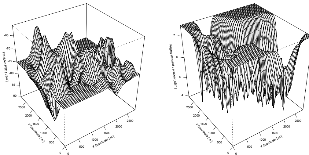
Fig. 6. Kriged estimates of the mean PSD field (left) and the standard deviations of the estimator (right) for the operator A data set.
