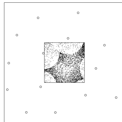
Fig. 3. Outcomes of 10^3 conditional simulation runs for the interior region of the data set of Figure 1 using the Strauss model for the node locations. The complex spatial structure of the conditional distribution is clearly visible.
