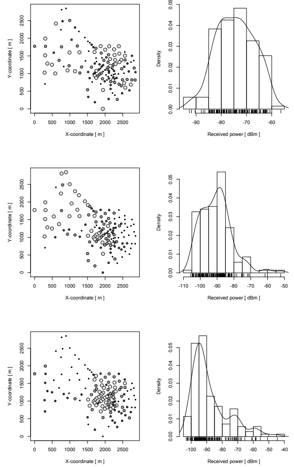
Fig. 4. Results from spatial spectrum use measurements for frequency bands of three cellular operators, denoted as operators A (top), B (middle) and C (bottom) in the following. Leftmost panels illustrate the spatial structure of the data sets while the rightmost panels show the marginal distributions of the data.
