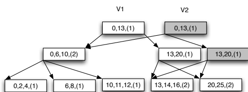
Figure 7: Node [13, 20] is cloned.
