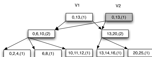
Figure 6: Creating a clone V2 of B+ tree V1.
