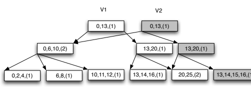
Figure 8: Leaf [13, 14, 16] is cloned. The new leaf is modified to host a new key 15.
