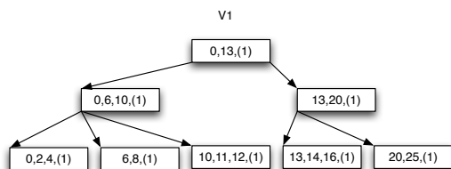
Figure 5: Initial B+ tree V1.
