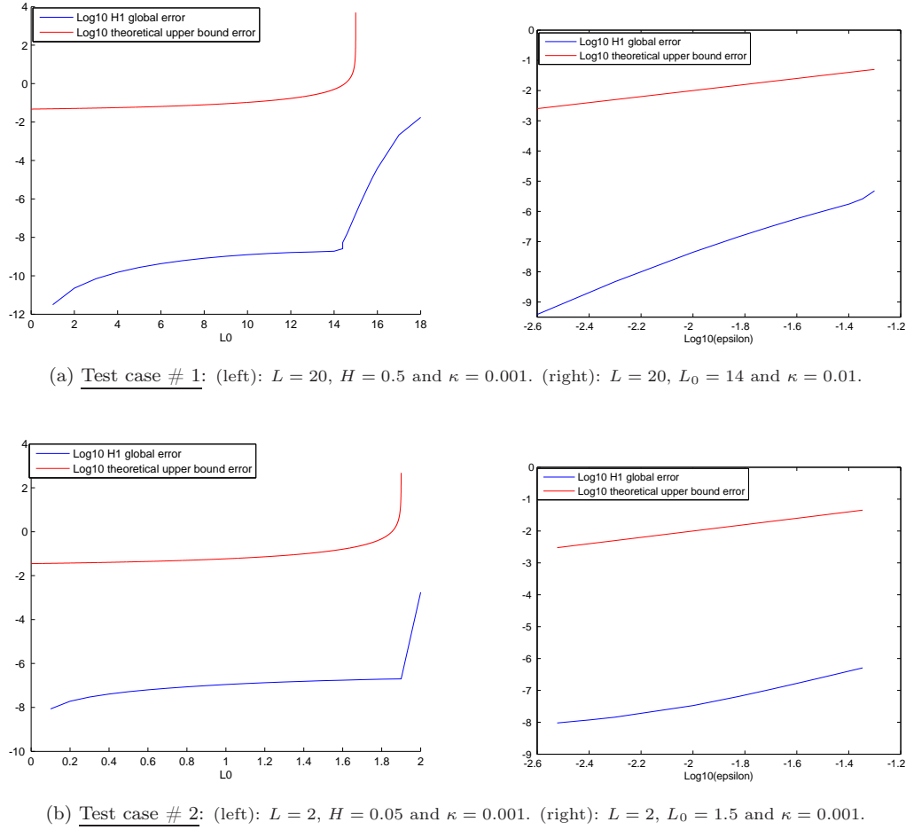
Figure 11: Relative error as a function of L_0 (left) and \epsilon (right) between the coupled solution and the 2-D reference solution in test case #1 (top) and #2 (bottom). In the left column, the red curves correspond (for both test cases) to the RHS of estimate (33).
