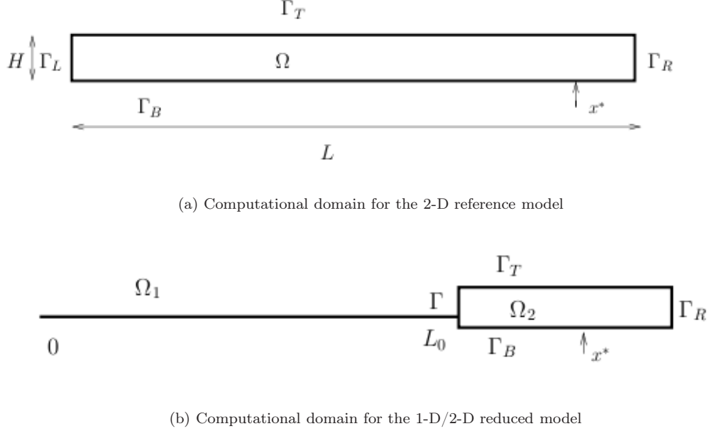
Figure 7: Computational domains for both the reference and reduced models in test case #1. For the reduced model (b), the 1-D/2-D interface \Gamma is located in x = L_0 .
