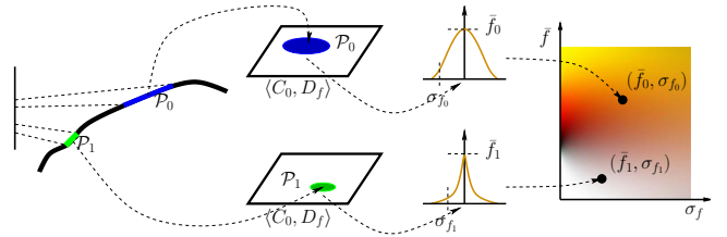
Figure 4: We prefilter the color map applied to a procedural function (e.g. noise). We sample specially constructed filtering distributions (right) using the function’s statistics over the surface patch.
