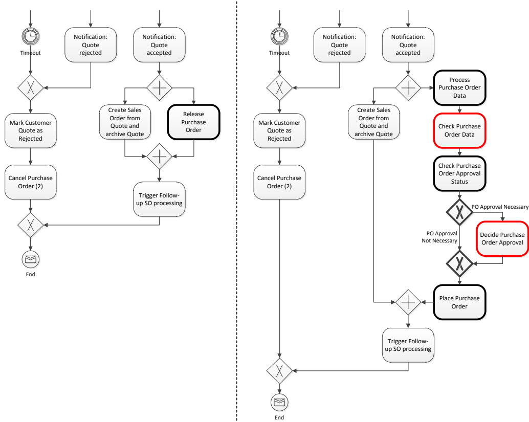
Figure 11: The BPMN process snippet from the screenshot in Figure 10, before (left) and after (right) calling the planner. The affected steps are highlighted in bold; actions with failed outcomes are highlighted in red as before.
