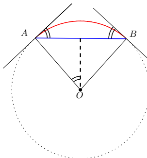
Figure 4: Property of angles.
