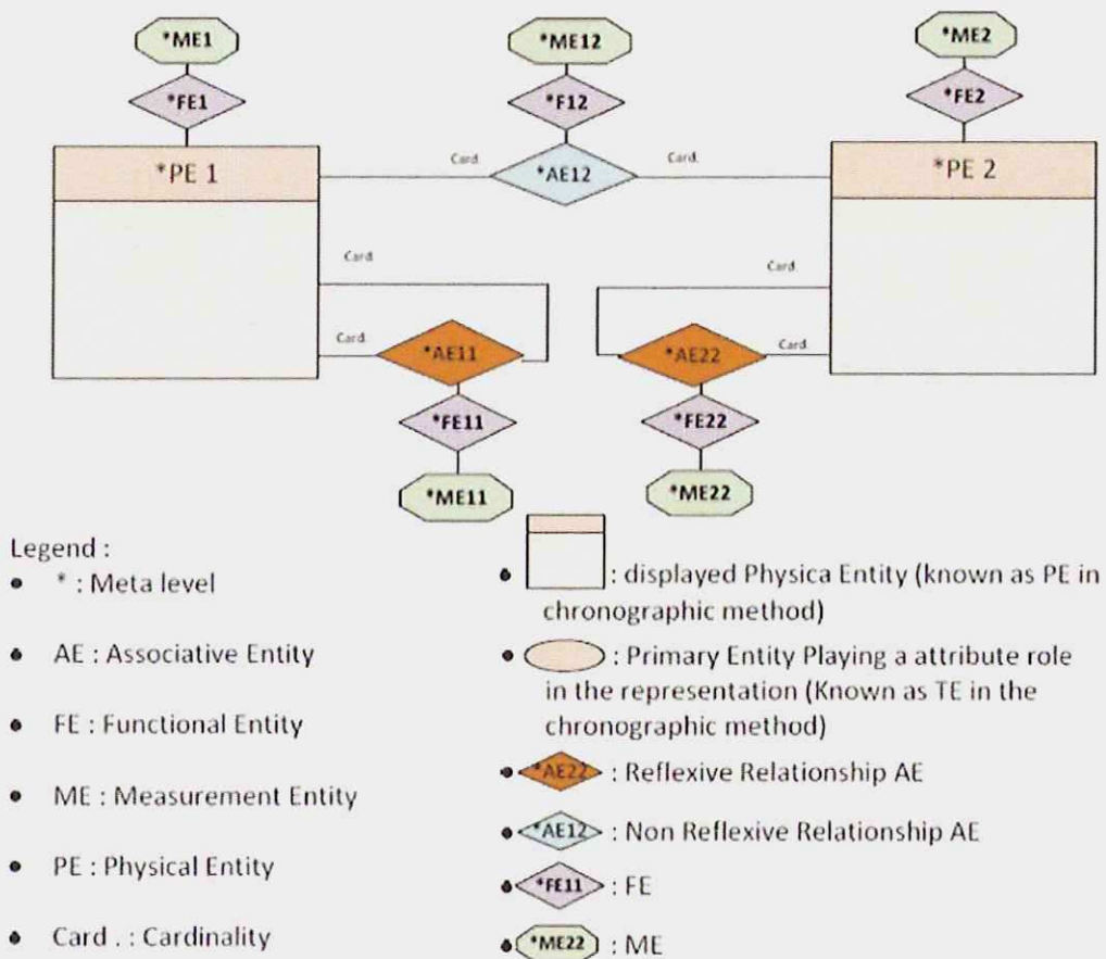
Figure 2: The meta-model
