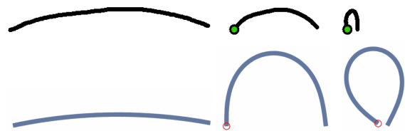
Figure 10: The method of [2] (top) compared to our approach (bottom). The rest shape (left) is edited by fixing the marked vertex and dragging the free end parallel to the horizontal line. Note that our approach does not suffer from the severe shrinkage noticeable on top.
