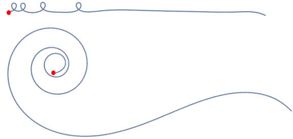
Figure 3: Illustration of the robustness of our approach to multiple loopings (top) and large rotations (bottom) where the user drags the free end in circular manner.
