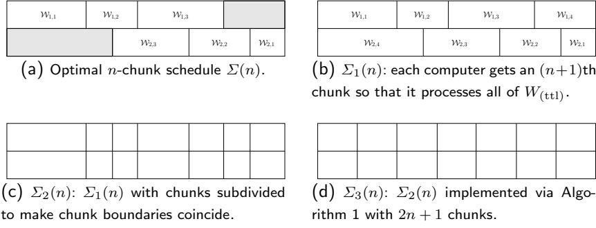
Fig. 2 Schedule transformations used to prove asymptotic optimality results in Theorems 6 and 8 (Algorithm 1 when W_{(\text{ttl})} \leq X ).
