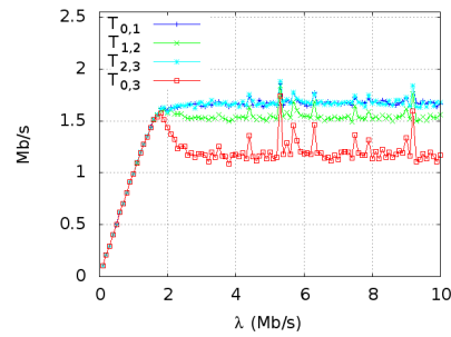
(a) Aggregate throughput on both directions for each link and for the overall network
