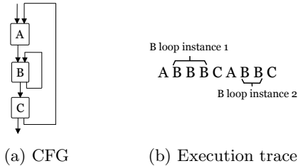
Figure 2: Simplified nested loop example
