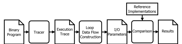
Figure 8: Aligot architecture
