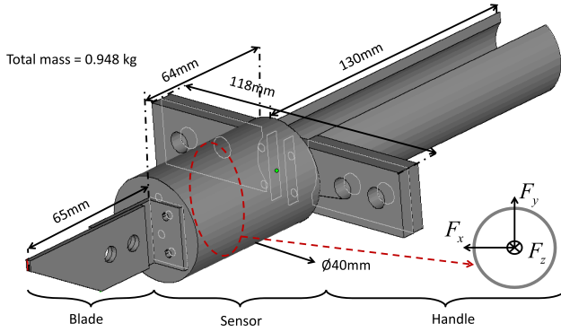
FIGURE 3. INSTRUMENTED KNIFE.
