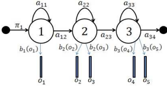
Fig. 1. Topology of the context-independent phonetic HMM.
