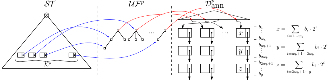
FIGURE 1. The simplicial complex is represented by a simplex tree \mathcal{ST} (left). The annotation vectors, represented as sequences of integers coded on w_b bits, are maintained in a dictionary \mathcal{D}_{\text{ann}}^p (right). \mathcal{UF}^p connects the p -simplices in \mathcal{ST} to their annotation vector in \mathcal{D}_{\text{ann}}^p (middle).
