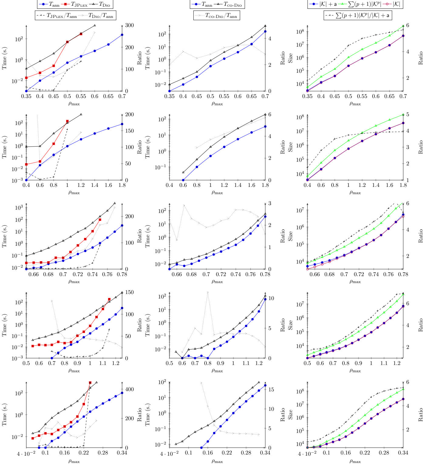
FIGURE 3. Left column: comparison of time performance between our implementation ( T_{\text{ann}} ), and the computation of persistent homology with JPLEX ( T_{\text{JPLEX}} ) and DIONYSUS ( T_{\text{Dio}} ). Middle column: comparison of time performance of our implementation ( T_{\text{ann}} ) and the computation of persistent cohomology in DIONYSUS ( T_{\text{co-Dio}} ). Right column: comparison of the memory performance of our implementation |\mathcal{K}| + \text{ann} with the sparse matrix representation \sum(p+1)|\mathcal{K}^p| . From Top to Bottom: Rips complex for 507 points from S4 , 1000 points from Bud , 500 points from Bro , 500 points from Cy8 and 4900 points from Kl .
