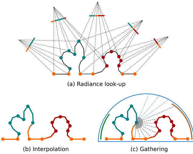
Fig. 4: Evaluation of sky and indirect illumination at each PMVS point. We look up the radiance value of the PMVS points in each image and average the values over the images where they are visible (a). We then project and interpolate this radiance over the proxy geometry (b). Finally we gather the sky and indirect illumination at each PMVS point by shooting rays which sample the hemisphere (c, dotted lines). Rays that reach sky pixels in the environment map (c, blue lines) contribute to sky illumination, while other rays contribute to indirect illumination (c, dark lines).
