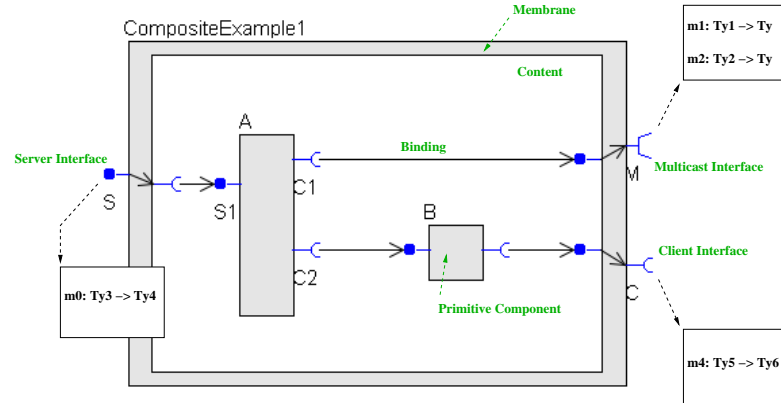
Figure 1: A typical GCM assembly
