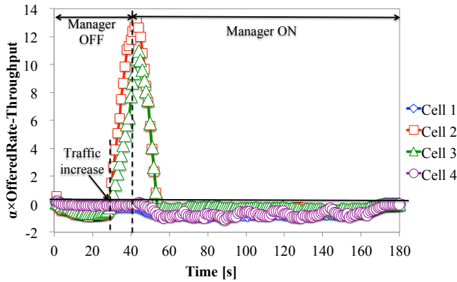
Figure 13. \alpha \times \sum_{STAs} OfferedRate_{STAs} - \sum_{STAs} PacketThroughput_{STAs} at each cell. The figure shows that the parameter reacts well to buffer overflow.
