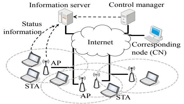
Figure 6. Besides having user-owned APs and STAs, the target community network has a centralized control manager. The information that are necessary for network management is collected by APs and/or STAs and gathered at an information server.
