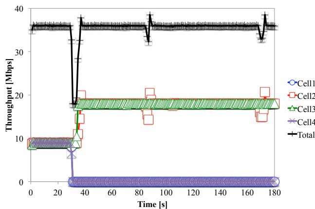
Fig. 17. Throughput performance of the cell aggregation mechanism. STAs at cells 1 and 4 are moved to cells 2 and 3.
