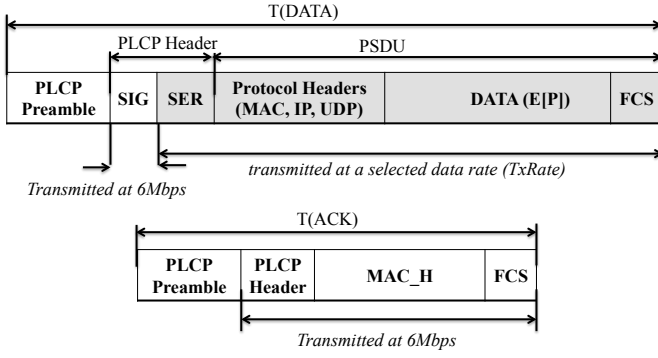
Fig. 3. T' the sum of the times required for transmissions of a data frame and the corresponding acknowledgment frame. PLCP SIGNAL field duration and ACK frame are generally coded with 1/2 BPSK (i.e., 6 Mbps rate) in the IEEE 802.11a systems. The shaded area of the data frame is transmitted at a rate ( TxRate ) selected by the MAC rate adaptation mechanism.
