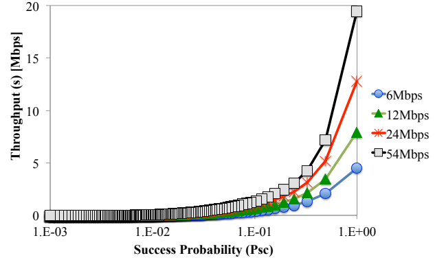
Fig. 4. The throughput performance as a function of the success probability. The figure shows that for a sufficient throughput is achieved only when the success probability is large.
