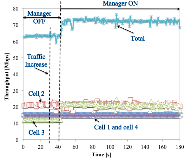
Fig. 14. Throughput performance of each cell. In this scenario, TCP and UDP traffic share the same resource at Cell2. Upon activation of the manager, a STA with UDP traffic is moved to Cell3. With this association control, more than 10 Mbps throughput improvement is achieved.
