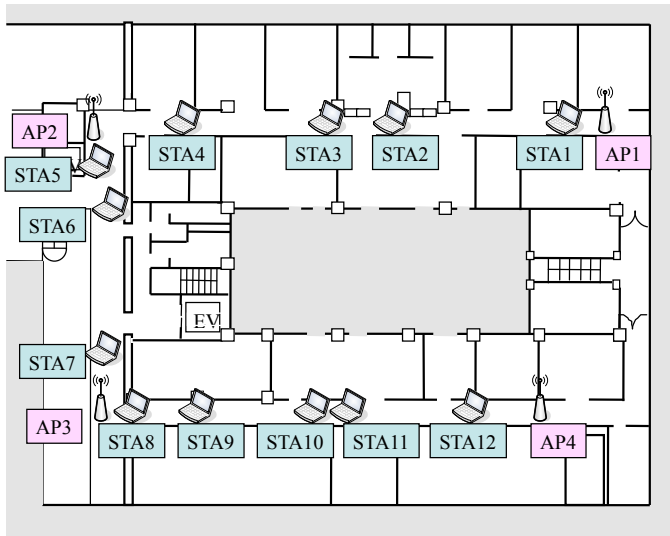
Fig. 9. An active office area, which has a complicated room and obstacle structure and intermittent movement of people, is used as the test environment. The test scenario consists of 4 APs and 12 STAs. STAs are initially associated with the APs using the strongest RSSI method.
