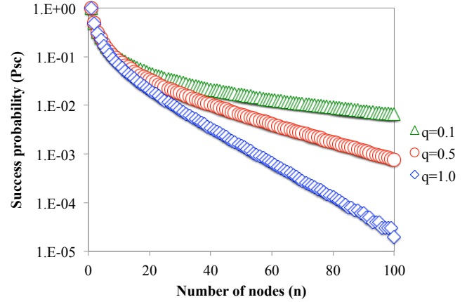
Fig. 2. Success probability as a function of the number of contending nodes. The figure shows that P_{sc} sharply decreases with the increase of the number of nodes. The smaller the probability of having a pending frame ( q ), the larger is the P_{sc} .
