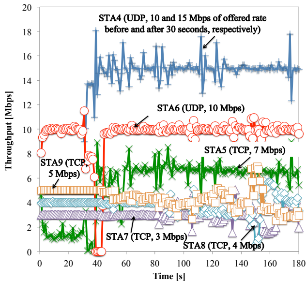
Fig. 15. Throughput of individual STAs at cells 2 and 3. Upon activation of the manager, STA6 is moved from Cell2 to Cell3. This enables TCP traffic at STA5 to increase its rate up to its maximum rate and the UDP traffic at STA4 also achieves its maximum throughput.
