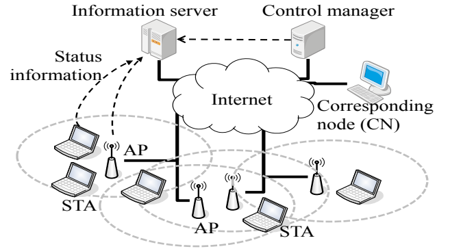
Fig. 6. Besides having user-owned APs and STAs, the target community network has a centralized control manager. The information that are necessary for network management is collected by APs and/or STAs and gathered at an information server.
