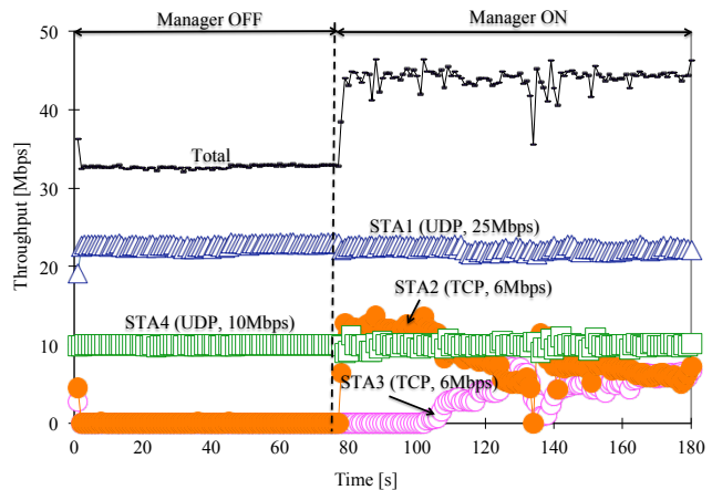
Fig. 16. Throughput of individual STAs for a scenario where STAs with TCP traffic are moved (STA2 and STA3). The TCP traffic could achieve increased throughput at the destination cell.
