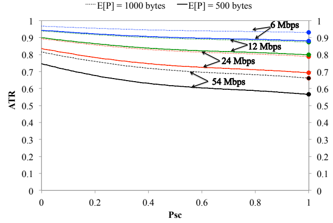
Fig. 5. ATR characteristics with respect to the success probability, P_{sc} . Note that the solid (dashed) lines correspond to 500 bytes (1000 bytes) of data size. The figure clearly shows that ATR is maximized when P_{sc} is minimized. The optimal value of ATR (that maximizes P_{sc} ) is smaller than the maximum value of ATR. The figure also shows that the larger the data rate, the smaller is the ATR and the larger the data size, the larger is the ATR.
