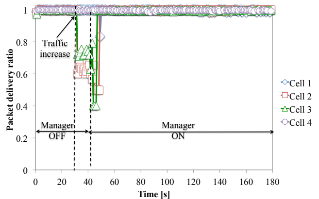
Fig. 11. Packet delivery performance of the congestion alleviation method. Due to the additional traffic injected after around 30 seconds, the packet delivery ratio largely degrades down to 60%. Upon activation of the manager, the delivery performance is recovered back to 100%.
