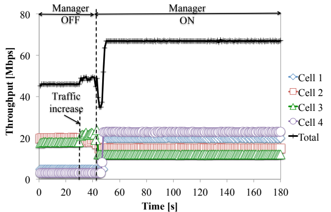
Fig. 10. Throughput performance of the congestion alleviation method. In this scenario all STAs have CBR/UDP traffic. Upon activation of the manager, STAs are moved from the congested cells (cells 2 and 3) to the non-congested neighboring cells (cells 1 and 4). The aggregate throughput is largely improved by the association control.
