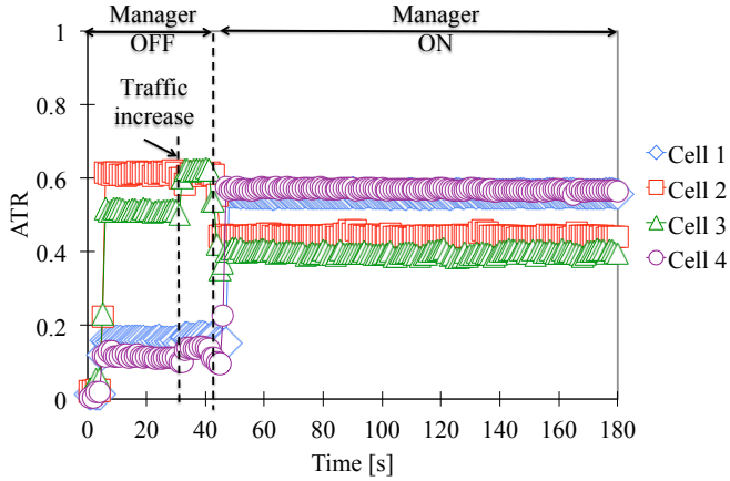
Fig. 12. ATR measured at each APs. The figure shows that ATR can be well tuned by the association control to the desired value.
