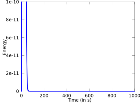
Fig. 3. Energy for \gamma = 0.249\kappa - y-scale magnified by 10^{10}
