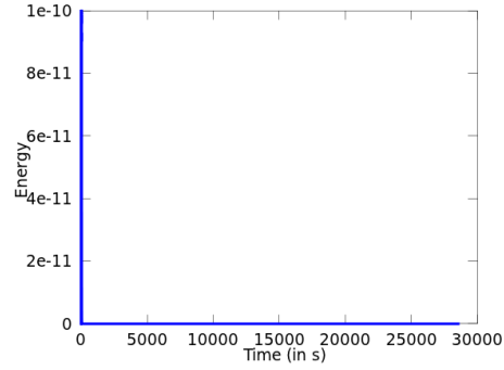
Fig. 5. Energy for \gamma = 0.249\kappa - y-scale magnified by 10^{10}
