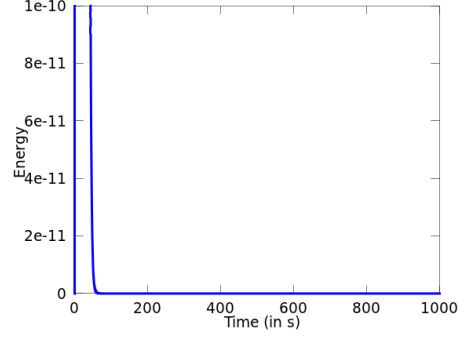
Fig. 3. Energy for \gamma = 0.249\kappa - y-scale magnified by 10^{10}
