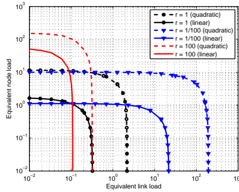
Figure 10: ER quadratic-linear comparison for p = 0.3 .
