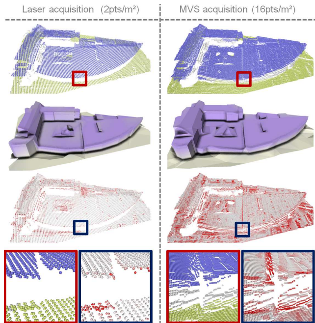
Fig. 17 Impact of the acquisition system type on our approach (from top to bottom) the classified point clouds, the obtained 3D-models, the input clouds with the points colored according to their distance to the associated 3D-models [color code: see Fig. 11], and some associated crops. The 3D-model from MVS is less accurate in terms of structure contouring, but is of similar quality concerning the surface recovery. The laser-based 3D-model (left) has a mean error to the input data slightly lower than the MVS-based 3D-model one (right), i.e. 0.26 m vs 0.33 m.
