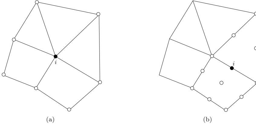
Figure 1: Illustration of the stencil for least square gradient recovery at the node i . The symbol (\bullet) indicates the node around which the Taylor series expansion is done while the symbols (\circ) indicate the node used to construct the least square problem. On the left stencil with linear elements, on the right stencil with quadratic elements for a nodes on the face.
