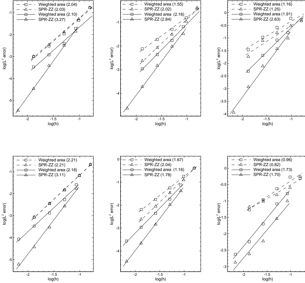
Figure 8: L^2 error in the solution of the linear advection-diffusion problem on quadrangular grids with linear (dashed lines) and quadratic (solid lines) elements. Error of the solution (first column), error of the x -component of the gradient (second column) error of the y -component of the gradient (third column). Linear scheme (upper), non-linear scheme (lower). In the legends are reported also the mean slopes of curves and h = 1/\sqrt{N_{\text{dof}}} .
