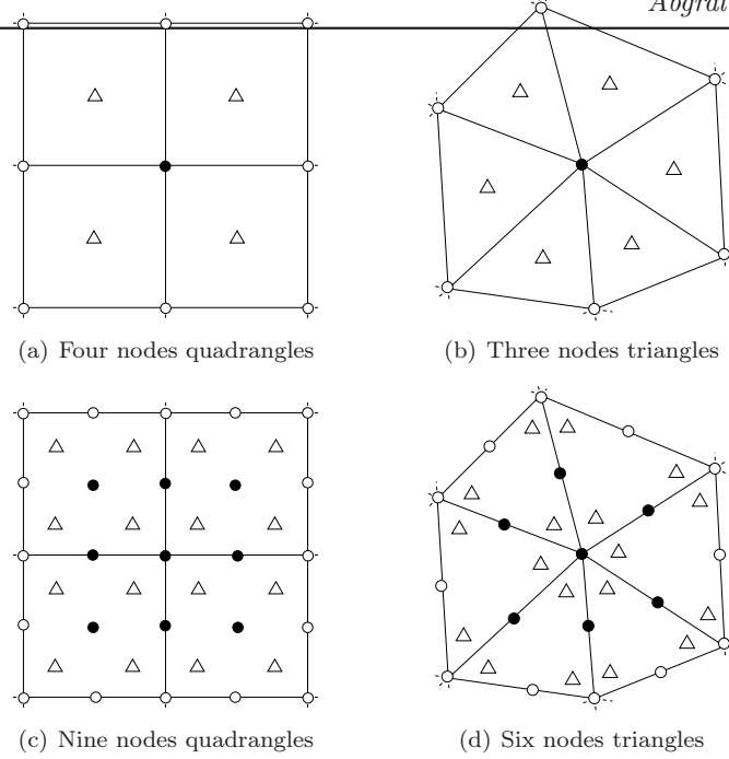
Figure 2: Interior super-convergent patches for quadrilateral and triangular elements: top linear elements, bottom quadratic elements. The symbols (o) indicate the patch assembly points, the symbols (●) indicate the points where the gradient is recovered and the symbols ( \Delta ) indicate the super-convergent sampling points.
