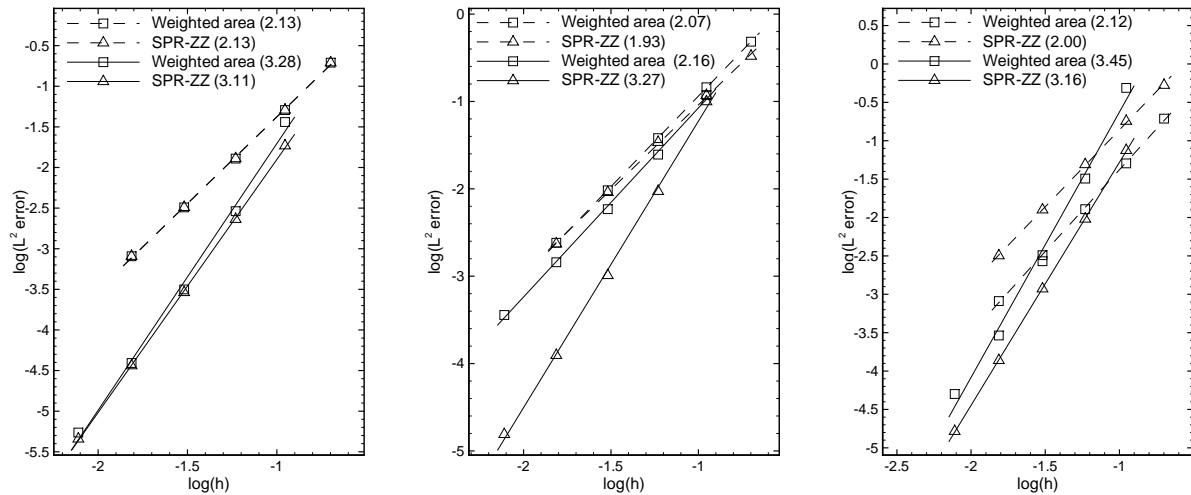
Figure 16: L^2 error in the solution of the anisotropic diffusion problem on uniform, structured grid of quadrangles, with linear (dashed lines) and quadratic (solid lines) elements. Error of the solution (first column), error of the x -component of the gradient (second column) error of the y -component of the gradient (third column). Linear scheme (upper), non-linear scheme (lower). In the legends are reported also the mean slopes of curves and h = 1/\sqrt{N_{\text{dof}}} .
