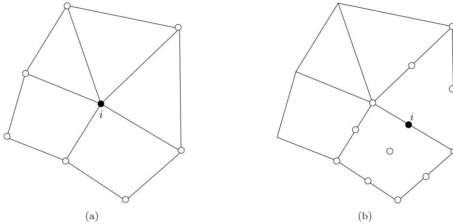
Figure 1: Illustration of the stencil for least square gradient recovery at the node i . The symbol (●) indicates the node around which the Taylor series expansion is done while the symbols (○) indicate the node used to construct the least square problem. On the left stencil with linear elements, on the right stencil with quadratic elements for a nodes on the face.
