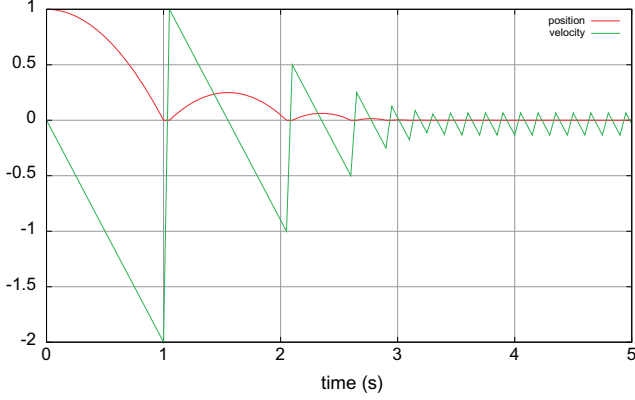
(a) Explicit position forecast (61) with \gamma = 0
