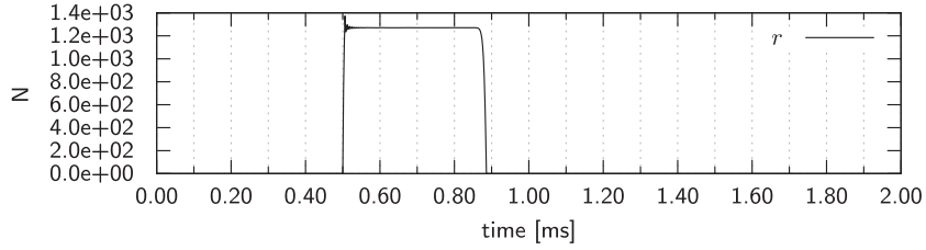
(b) Time-step h = 2 \times 10^{-6} s.
