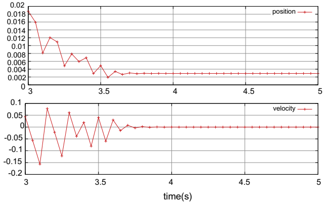
(b) Zoom on t \in [3, 5] with \theta = 1
