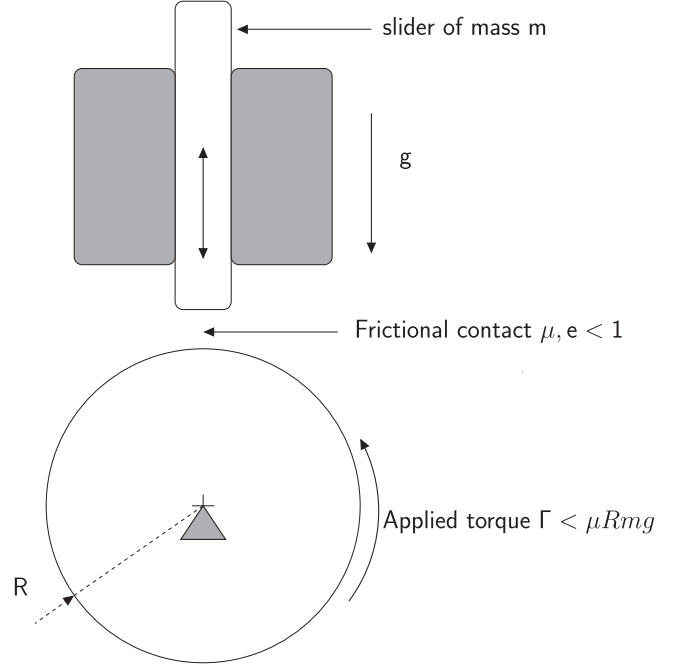
Fig. 8. A slider and roller example.
