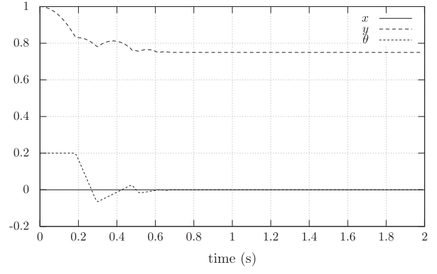
(b) Coordinates with Algorithm 2
