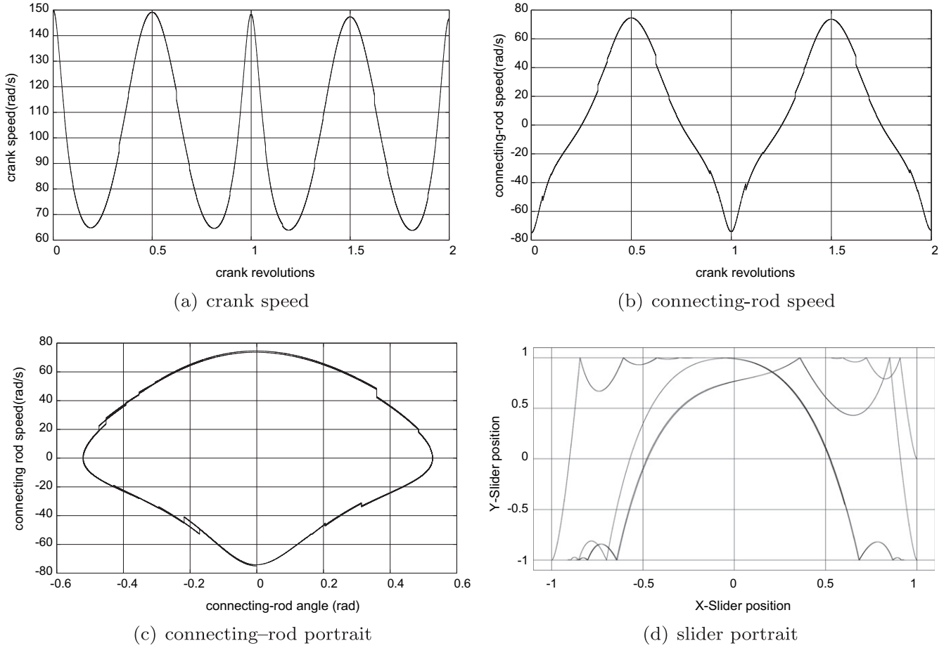
Fig. 21. Details of the motion of the slider-crank with the standard Moreau-Jean time-stepping scheme for h = 10^{-6} s.
