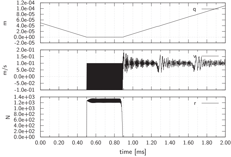
Fig. 11. Trapezoidal rule with a position-based constraints. Position q , velocity v and reaction force r at the contact point. h = 2 \times 10^{-6} s. Number of elements N = 1000 .
