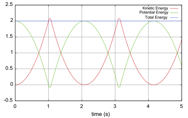
(b) Energy diagram \theta = 1/2 without projection
