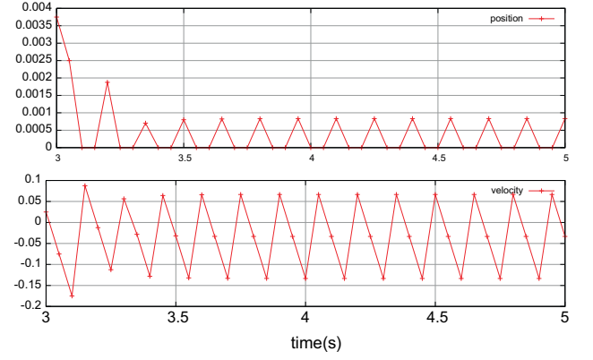
(b) Zoom on t \in [3, 5] for \gamma = 0
