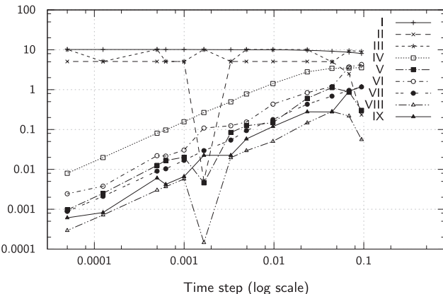
(c) The linear oscillator (Example 2). Velocity error
