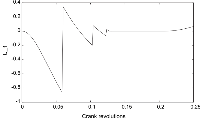
(a) Moreau-Jean's scheme (18d) on [0, 0.25] .
