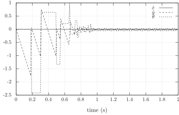
(c) Velocities with Algorithm 1
