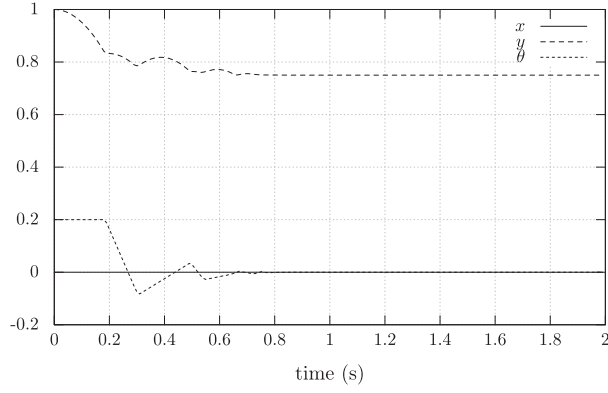
(a) Coordinates with Algorithm 1
