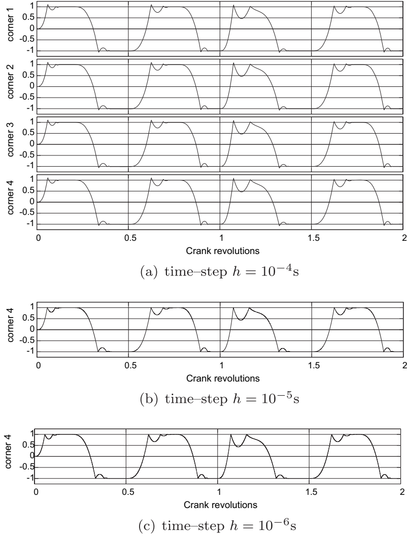
Fig. 22. Dimensionless motion of the slider corners with the standard Moreau-Jean time-stepping scheme for different time-steps.
