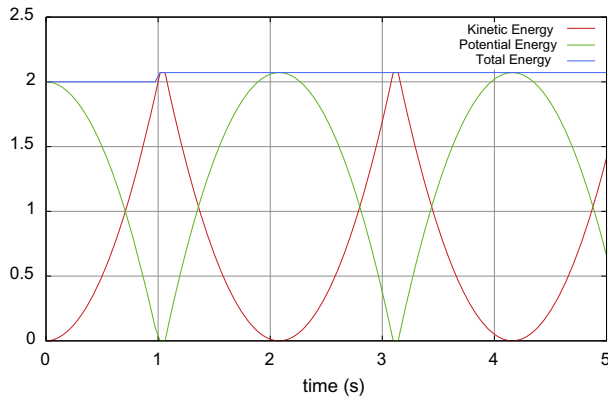
(a) Energy diagram \theta = 1/2 with projection
