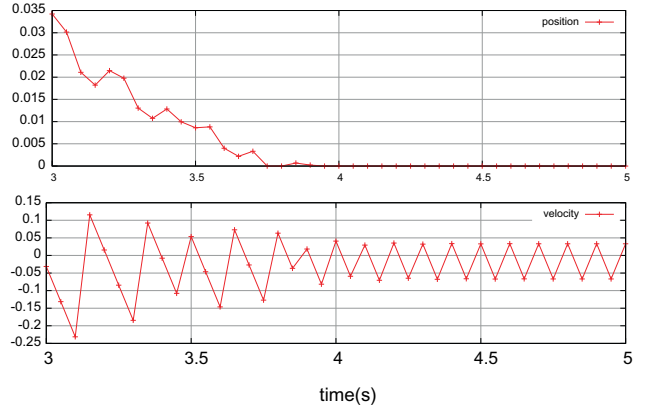
(f) Zoom on t \in [3, 5] for \gamma = 2
