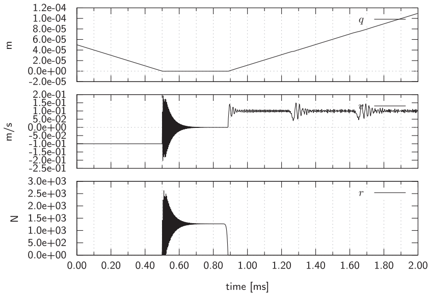
Fig. 15. Moreau-Jean's scheme with a restitution coefficient e = 0.95 . h = 2 \times 10^{-6} s. Number of elements N = 100 .
