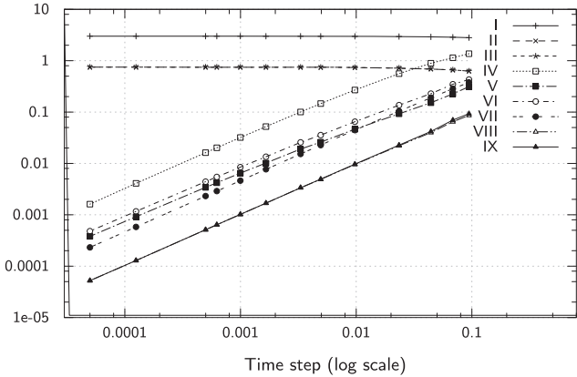
(a) The bouncing ball (Example 1). Velocity error
