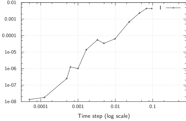
(a) The bouncing ball (Example 1). \max_k(\|\tau_k\|)
