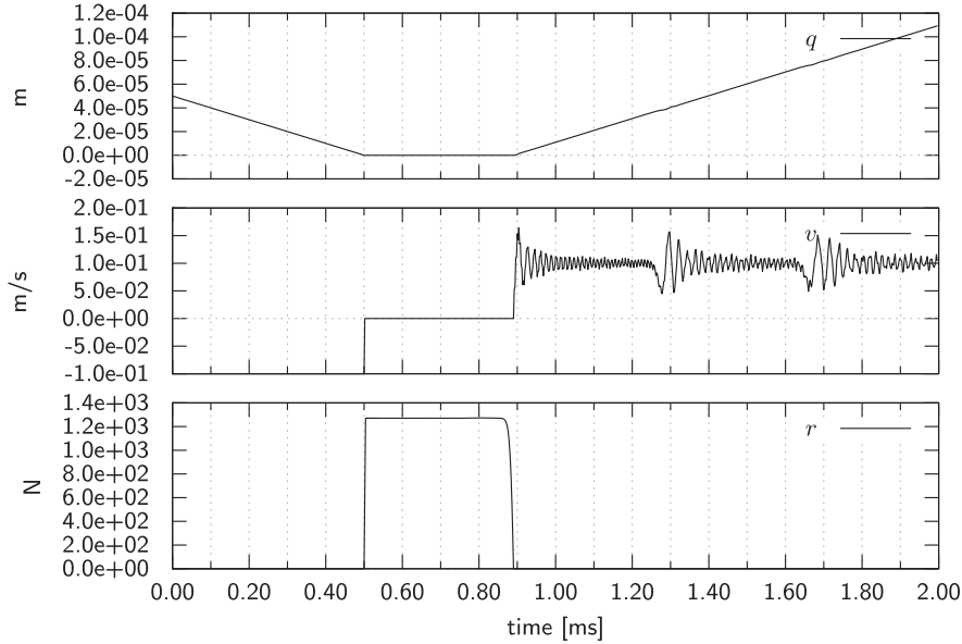
Fig. 12. Moreau-Jean scheme. Position q , velocity v and reaction force r at the contact point. \theta = 1/2 , h = 5 \times 10^{-5} s. Number of elements N = 1000 .
