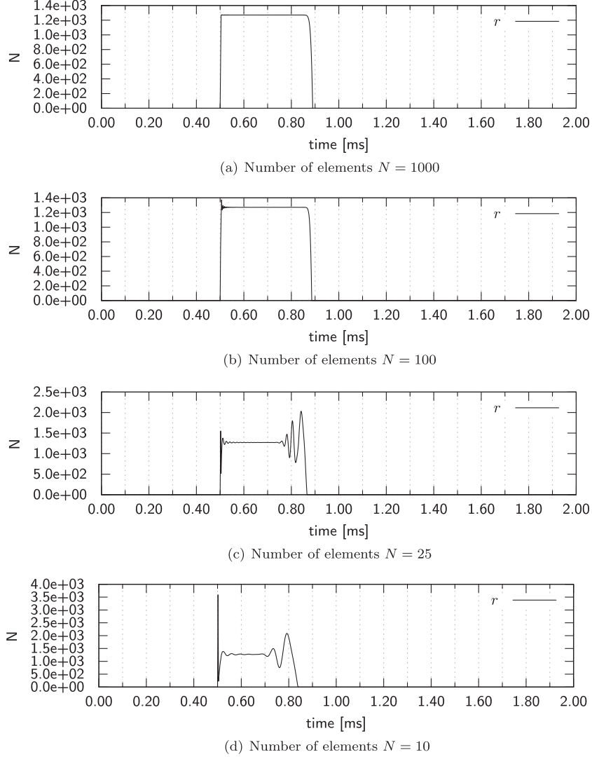
Fig. 13. Contact force r for Moreau–Jean’s scheme. \theta = 1/2 , h = 2 \times 10^{-6} s. Effect of the element length.
