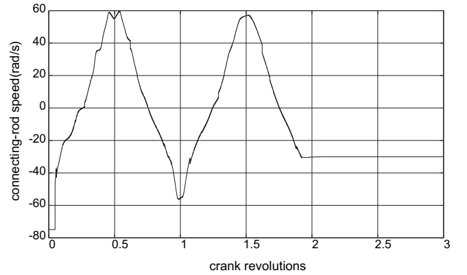
(b) connecting-rod speed
