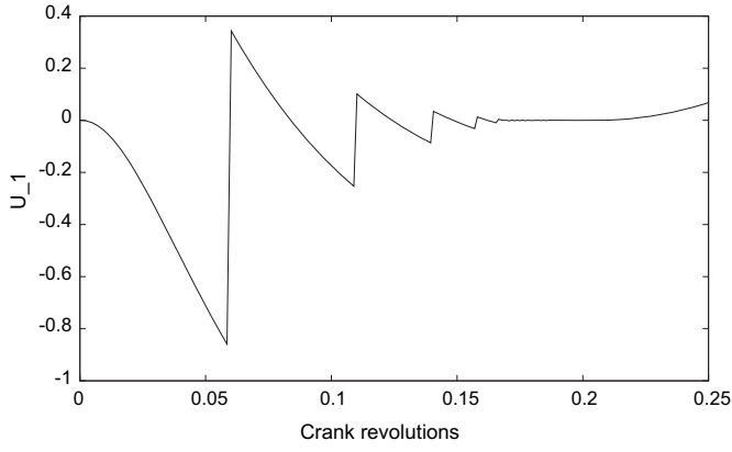
(c) Direct projected scheme (Algorithm 1) on [0, 0.25] .
