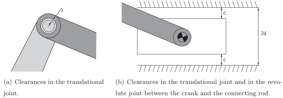
Fig. 20. Details of the clearance modeling.
