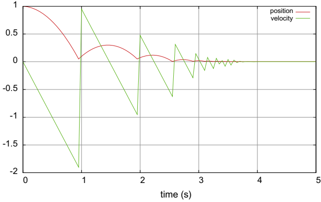
(a) Free position forecast (62) with \theta = 1
