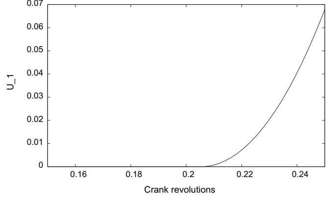
(b) Moreau-Jean's scheme (18d) on [0.15, 0.25] .
