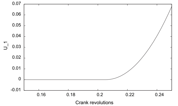
(f) Combined scheme (Algorithm 2) on [0.15, 0.25] .
