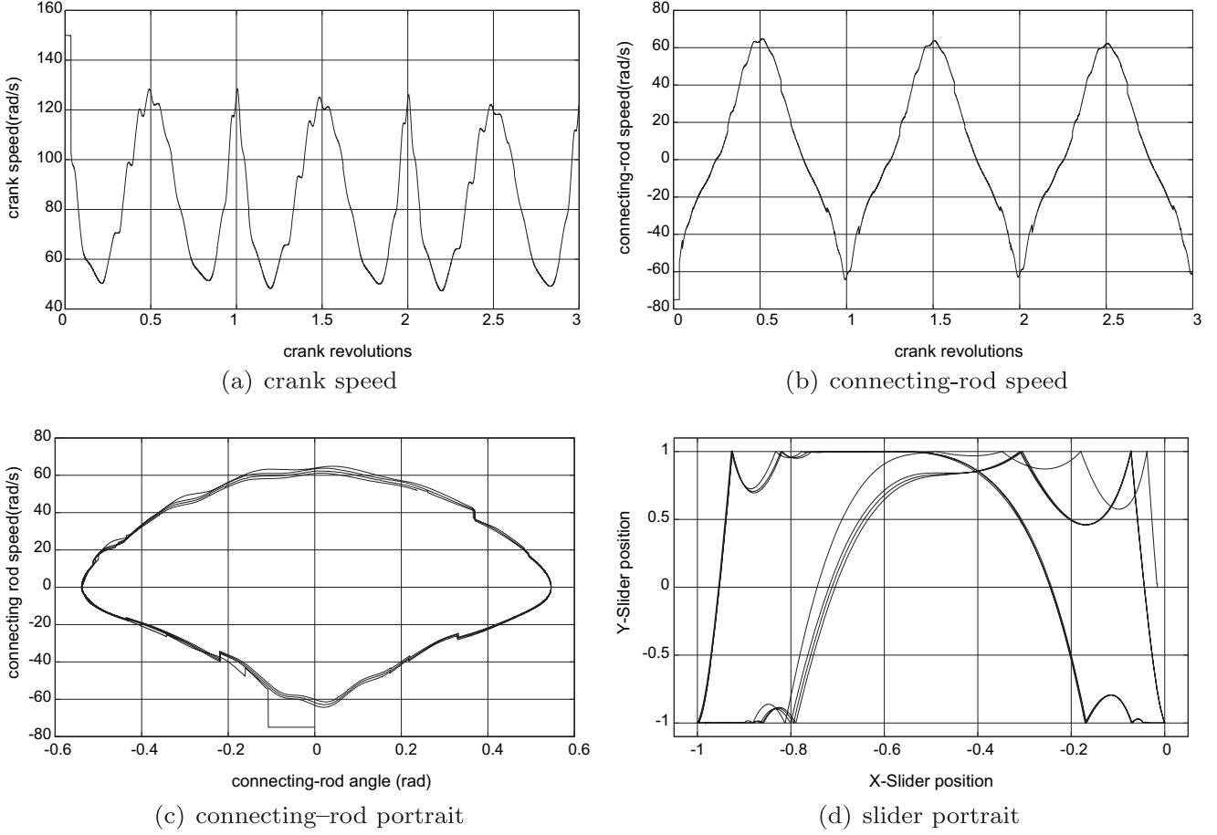
Fig. 28. Details of the motion of the slider crank with the combined projection time-stepping scheme for h = 10^{-05} s and a play in the revolute joint r = 5 \times 10^{-03} m.
