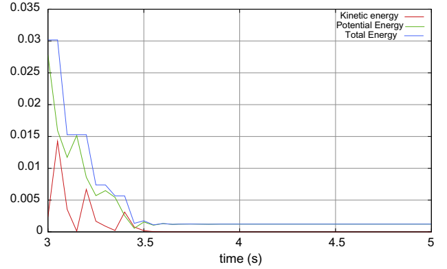
(d) Zoom on t \in [3, 5] Energy diagram with \theta = 1/2 . Free position forecast (62).
