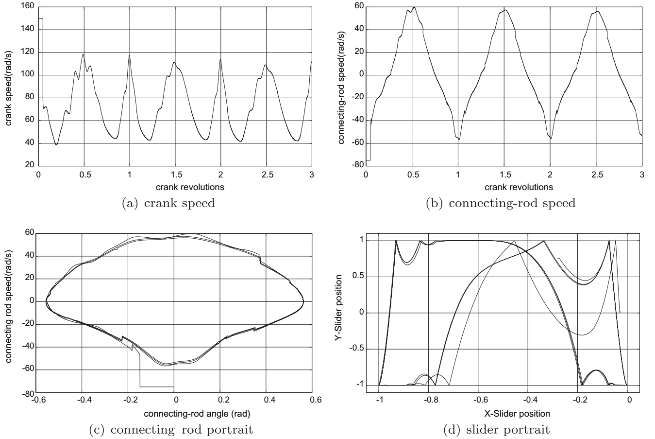
Fig. 27. Details of the motion of the slider crank with the combined projection time-stepping scheme for h = 10^{-5} s and a play in the revolute joint r = 5 \times 10^{-4} m.
