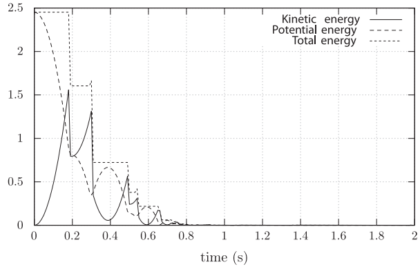
(e) Energies with Algorithm 1
