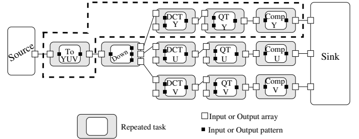
Fig. 1. Array-OL Specification of a JPEG encoder. A gray-scale JPEG encoder only contains the tasks enclosed by the dotted lines.
