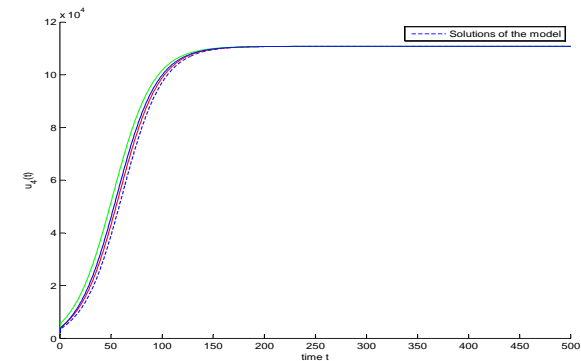
Figure 6: Trajectories of the infected populations with different initial conditions when \mathcal{R}_0 > 1
