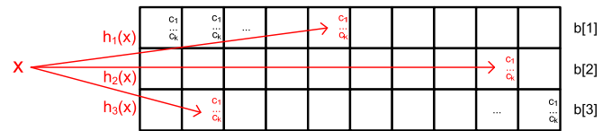
Figure 2. Count-min Sketch adapted for classification.
