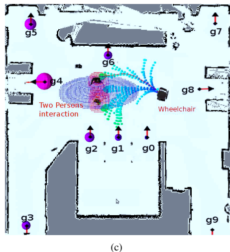
Fig. 8. Experimental scenario, in a) The wheelchair used for testing in b) the INRIA's hall. Possible goals are marked with a circle, the persons present in the scene are tracked by one of the Kinect sensors while the other Kinect is used to track the face of the user. c) Results of the system in a real scenario. The size of the spheres in the environment represent the value of the computed posterior probability for each destination. The computed trajectory and interaction regions are also shown.
