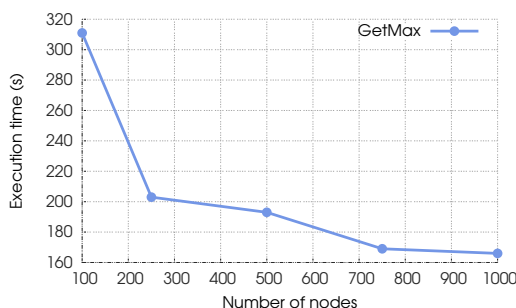
Figure 7: Execution time of GetMax containing 50,000 molecules.
