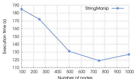
Figure 8: Execution time of StringManip with 20,000 molecules.
