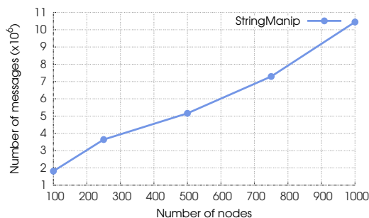
Figure 10: Number of messages sent during the execution of StringManip .
