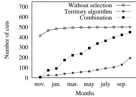
Figure 17: Number of optimality cuts at each time step
