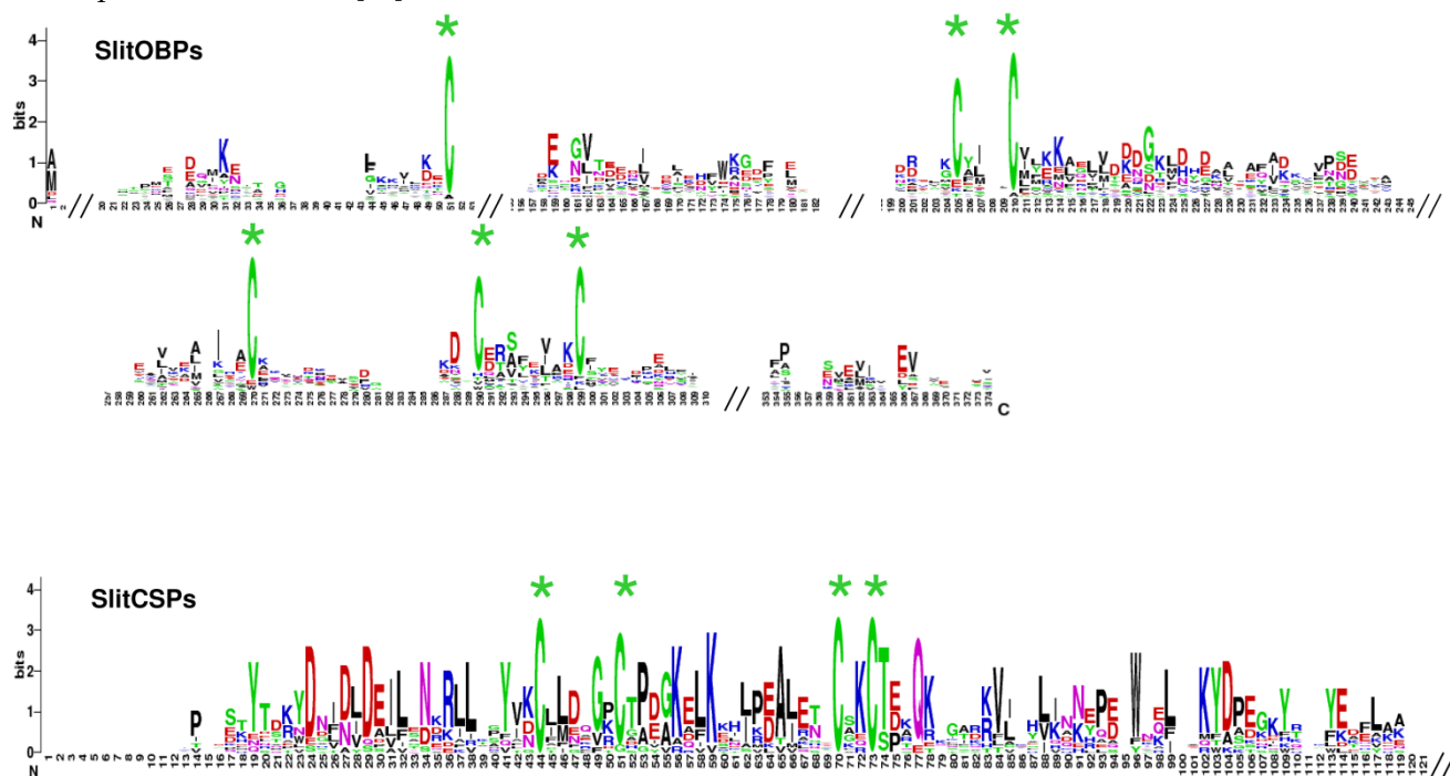
Figure 6. SlitOBP and CSP sequence logo. Degree of amino acid sequence conservation [38] along the primary sequence axis of odorant-binding proteins (OBPs) and the chemosensory proteins (CSPs) of S. littoralis . Depicted amino acid character size correlates to relative conservation across aligned sequences. Green asterisks indicate the conserved six and four cysteine motifs of OBP and CSP, respectively.
