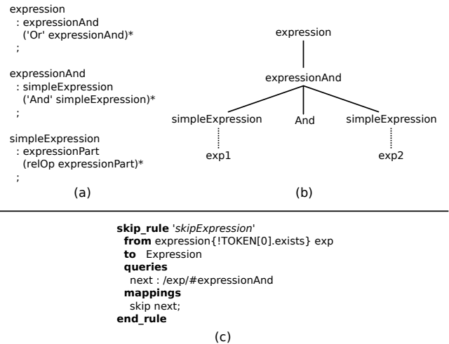
Fig. 10 (a) Grammar rules to parse both AND and OR expressions and (b) the corresponding syntax tree for the expression exp1 And exp2 . (c) Skip rule for the expression grammar element.
