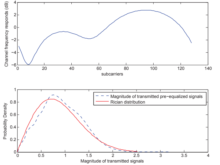
Fig. 4. Probability density of signals in a frequency flat fading WiMAX SUI channel
