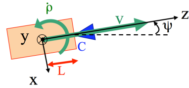
Figure 6: Model of the Cycab vehicle (Cycab can be seen on Figure 10).
