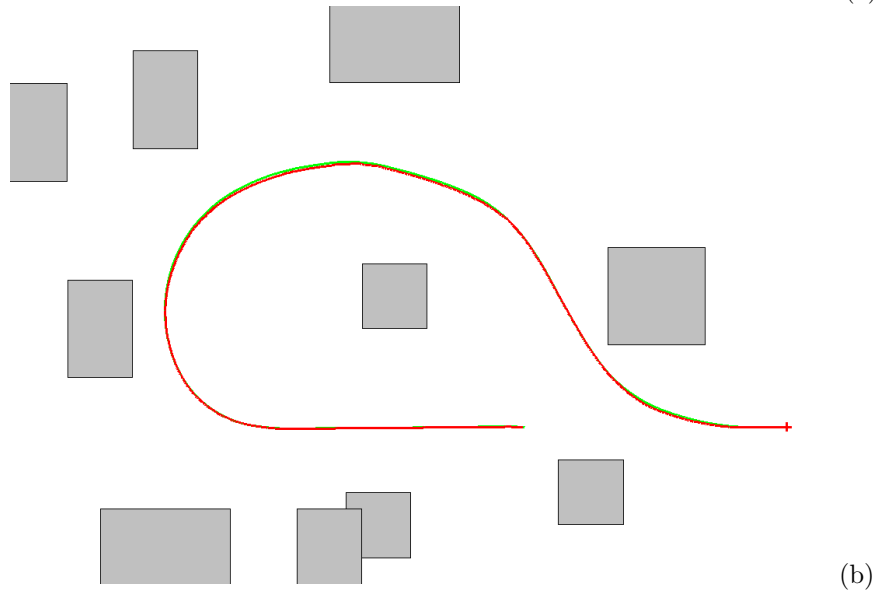
Figure 8: Simulation experiment. (a) Aerial view of the environment, (b) 2D representation of map with the learned trajectory in green and the resulting path in red (gray rectangles are buildings).
