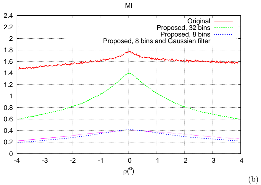
Figure 4: Method used to compute mutual information with respect to the rotation around the vertical axis \rho . (a) External view of the camera at the desired position in red (used to acquire the desired image \mathbf{I}^* ) and at the various positions of rotation in green. (b) shows the computed mutual information between \mathbf{I}(\rho) and \mathbf{I}^* with respect to the rotation \rho computed using various formulation.
