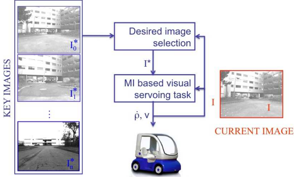
Figure 2: Navigation based on multiple visual servoing tasks.
