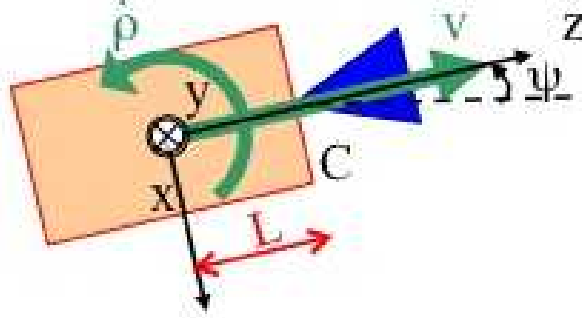
Figure 6: Model of the Cycab vehicle (Cycab can be seen on Figure 10).
