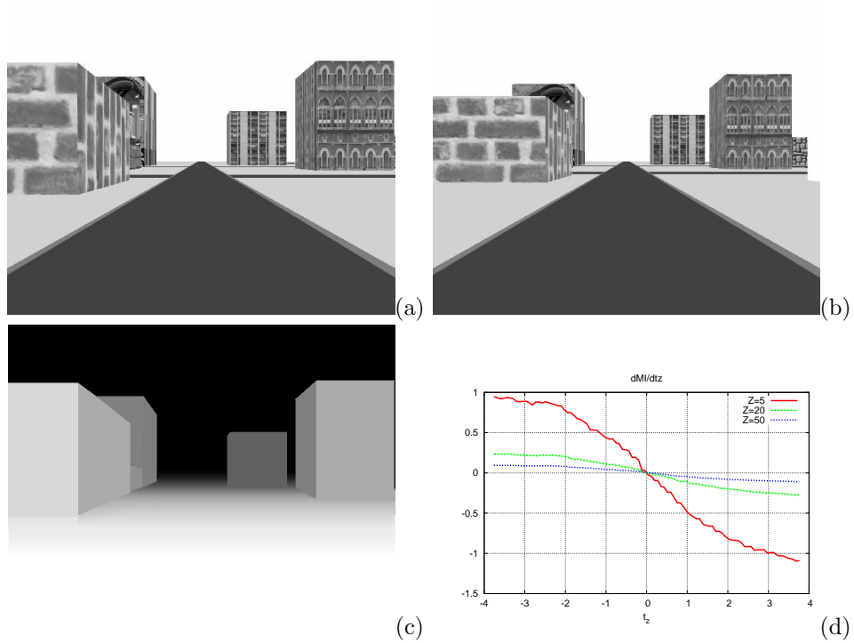
Figure 7: Translation estimation between the current and desired image. (a) Desired image, (b) acquired image with a 4 meter translation, (c) scene depth and (d) derivative of mutual information with respect to the translation along the z axis (in meters) with various fixed scene's depth Z .
