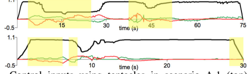
Fig. 4. Control inputs using tentacles in scenario A.1 (top) and A.2 (bottom): v (black, in \text{ms}^{-1} ), \omega (green, in \text{rads}^{-1} ), and \dot{\varphi} (red, in \text{rads}^{-1} ). The iterations with strong H are highlighted in yellow.
