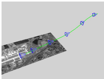
Fig. 12. From the homography to the estimation of the camera position. Green curve: estimated camera trajectory in the 3D space, blue: the 6 estimated camera positions corresponding to the frames represented in figure 13.
