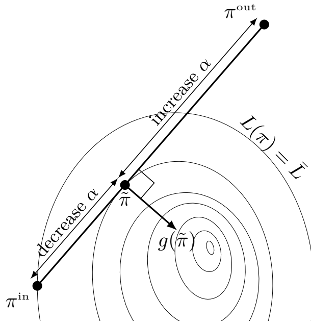
Fig. 6: Auto-adaptive \alpha -schedule: condition for increasing or decreasing \alpha depending on whether the \pi^{\text{sep}} is below or beyond the threshold value \tilde{\pi} .
