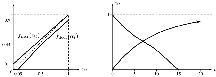
Fig. 5: Functions for increasing and decreasing \alpha are presented on the left side. The right side shows how the value of \alpha changes when \alpha increases or decreases on each iteration using these functions.
