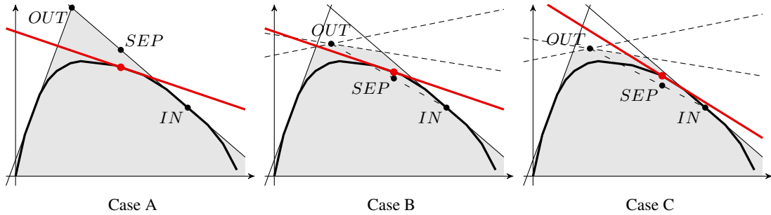
Fig. 2: The three cases that can arise when attempting to cut point (\pi^{sep}, \eta^{sep}) . Case A: (\pi^{sep}, \eta^{sep}) is cut-off by z^t . Case B: (\pi^{sep}, \eta^{sep}) is not cut but (\pi^{out}, \eta^{out}) is. Case C: neither (\pi^{sep}, \eta^{sep}) , nor (\pi^{out}, \eta^{out}) are cut, which results in a mis-pricing .
