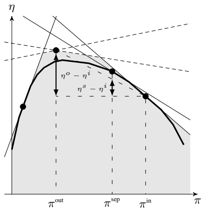
Fig. 4: In the case where (\pi^{sep}, \eta^{sep}) cannot be cut, then (L(\pi^{sep}) - \eta^{in}) \geq (\eta^{sep} - \eta^{in}) = (1 - \alpha)(\eta^{out} - \eta^{in}) , as outlined in Proposition 1-(ii).
