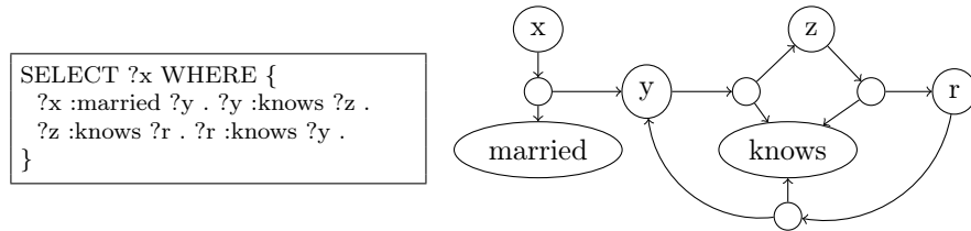
Figure 1: Cyclic query
