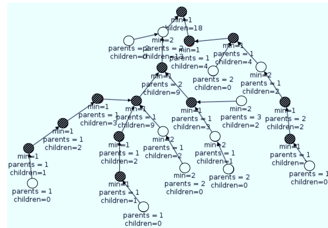
(b) Sparse-Loss
