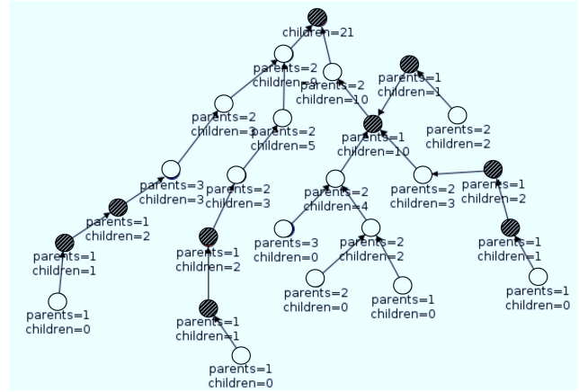
(b) Sparse-Loss
