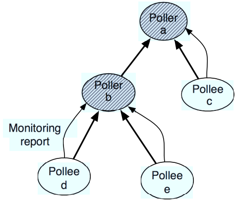
Fig. 1. An example of poller-pollee structure.
