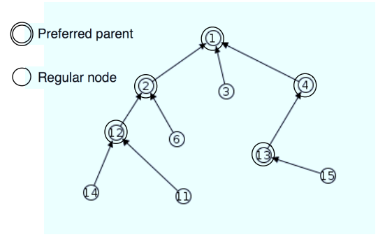
Fig. 2. RPL DODAG architecture.
