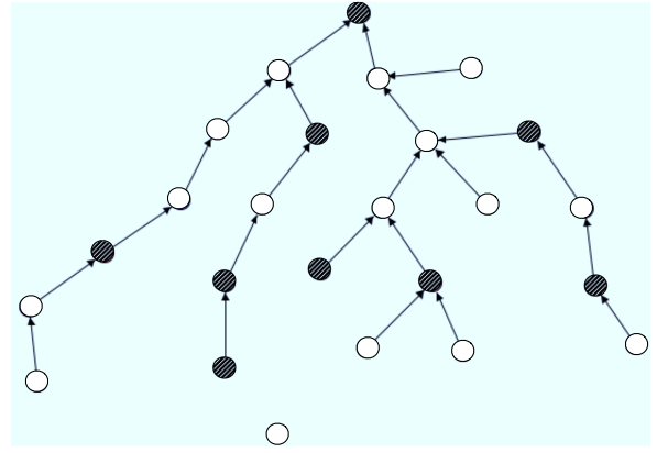
Fig. 11. A snapshot of the poller-pollee distribution after running the hybrid algorithm [2] where k_1 = k_2 = 1 .
