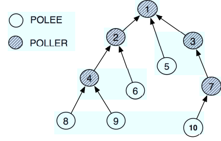
Fig. 3. A Poller-Pollee deployment using a trivial algorithm where all parents are POLLERS.
