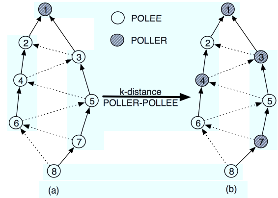
Fig. 6. Illustration of a Poller-Pollie deployment using the proposed algorithm 1. In (a), the distance between the poller 1 and the pollee 8 is equal to 3. (b) represents the resulting placement after applying the k -distance POLLER-POLLEE rule, where k is equal to 1.
