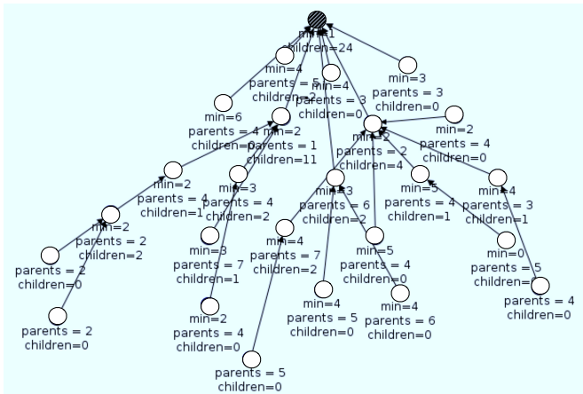
Fig. 8. A snapshot of the poller-polllee distribution after running the critical-parent strategy on a dense network.
