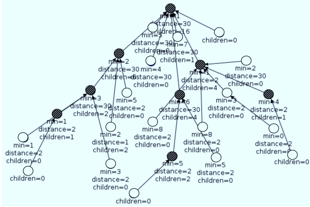
Fig. 10. A snapshot of the poller-pollee distribution after running the parent-articulation strategy and the k -distance rule on a dense network. k = 1 .
