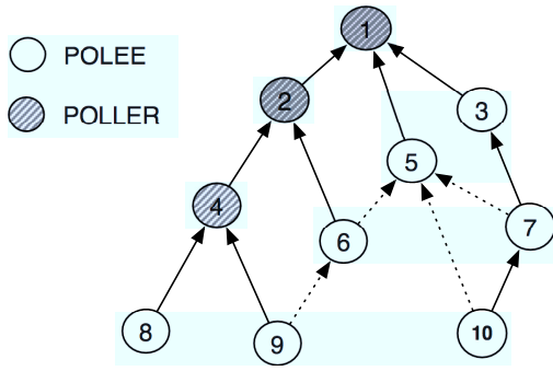
Fig. 4. A Poller-Pollie deployment using the critical-parent algorithm. Solid lines represent link to the selected parent and dashed lines represent back links to candidate parents.
