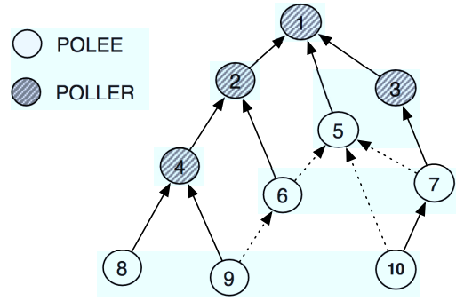
Fig. 5. A poller-pollie deployment using the critical link strategy. Solid lines represent link to the selected parent and dashed lines represent back links to candidate parents.
