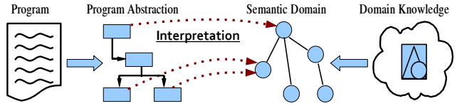
Figure 4. Framework for assigning (domain) meaning to programs
