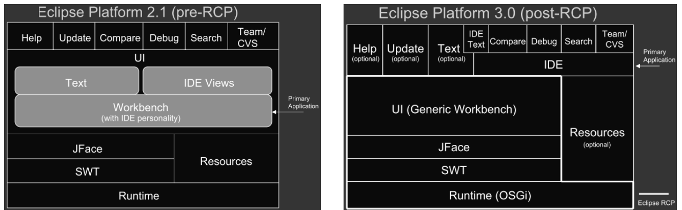
Fig. 1. An illustration of the architecture of the Eclipse platform before RCP (v. 2.1) and after RCP (v. 3.0). From a presentation at EclipseCon 2004.
